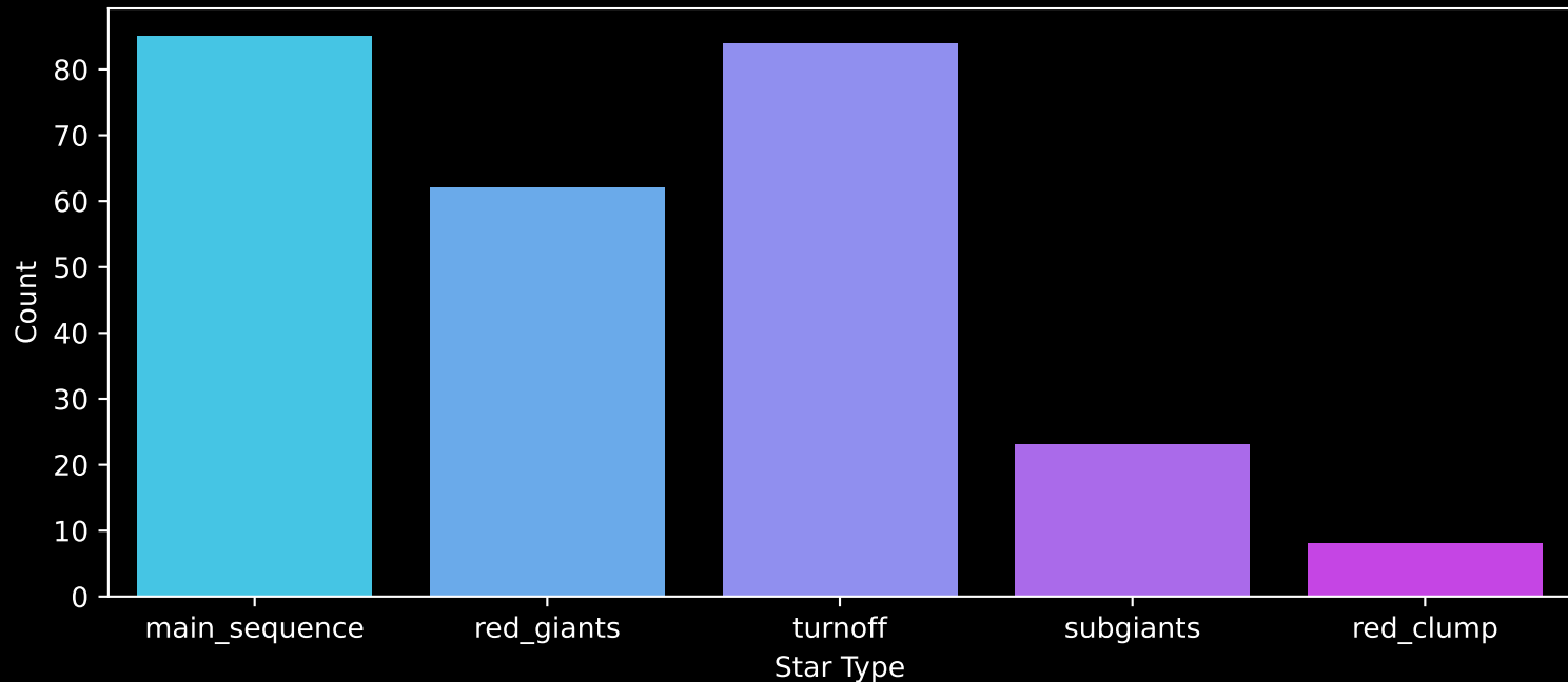
GALAH DR4 Field: [2930] Count plot of Star Type
