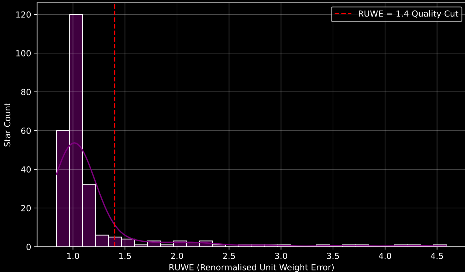
GALAH DR4 Field [2930] RUWE Distribution (n= 251)
